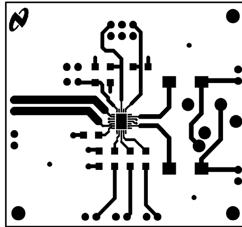
Recommended LQ PC Board Layout: Top Layer
