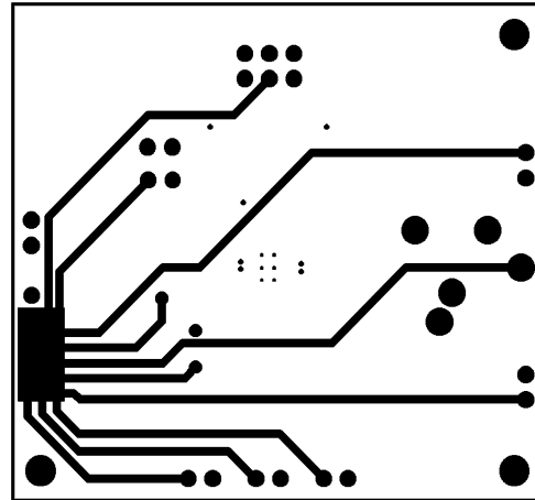
Recommended LQ PC Board Layout: Middle 2 Layer
