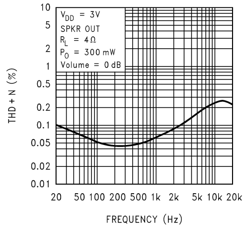
THD+N vs Frequency LM4852LQ
